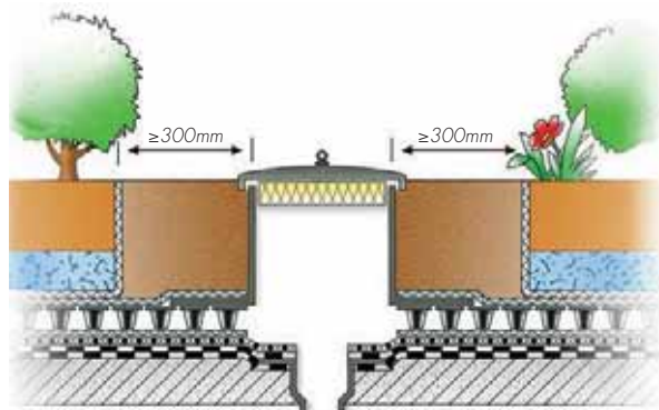
Detail 5. Roof outlet
