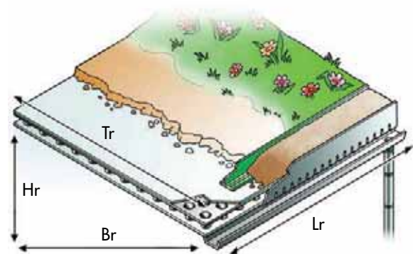
Figure 1. Roof dimensions
