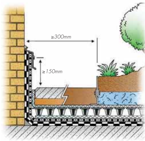
Detail 2. Facade
