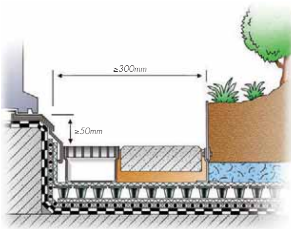
Detail 4. Door threshold
