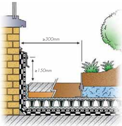
Detail 3. Facade with an opening
