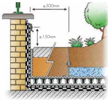
Detail 1. Parapet
